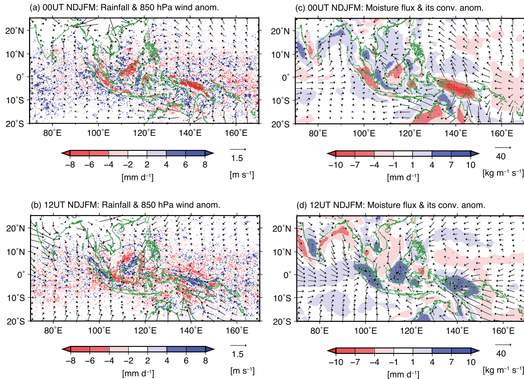
FIG. 7. (a),(b) Climatological (1998–2012) mean anomalies of TRMM-PR precipitation ( \text{mm day}^{-1} ; shaded areas) and wind vectors ( \text{m s}^{-1} ) at 850 hPa at 0000 UTC and 1200 UTC in NDJFM. (c),(d) As in (a) and (b), but for vertically integrated moisture flux vectors ( \text{kg m}^{-1} \text{s}^{-1} ) and convergence ( \text{mm day}^{-1} ; shaded areas). The climatological daily mean at each grid point has been removed.
