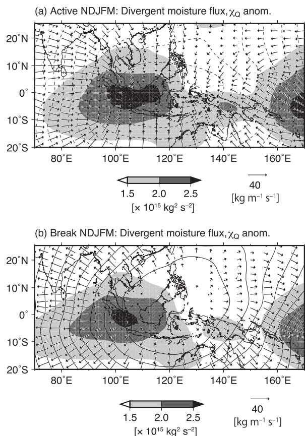
FIG. 9. Composite anomalies of the vertically integrated moisture flux potential ( \text{kg m}^{-1} \text{ s}^{-1} ; contours) and divergent moisture flux vectors ( \text{kg m}^{-1} \text{ s}^{-1} ) of vertically integrated moisture fluxes in peak (a) active and (b) break phases. These anomalies show the difference from the seasonal mean (NDJFM). The shading also indicates the composite variance in the diurnal component of the moisture flux potential between both phases. The solid (dashed) contours show positive (negative) values. The contour interval is 1 \times 10^8 \text{ kg s}^{-1} , from -1.2 to 1.3 \times 10^8 \text{ kg s}^{-1} . Vectors, contours, and shading are plotted only if significant at the 95% confidence level.
