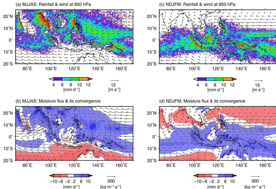
FIG. 1. Climatological (1998–2012) mean distributions of (a) TRMM-PR precipitation ( \text{mm day}^{-1} ; shaded areas) and wind vectors ( \text{m s}^{-1} ) at 850 hPa and (b) vertically integrated moisture (from the surface to 100 hPa) flux vectors ( \text{kg m}^{-1} \text{s}^{-1} ) and its convergence ( \text{mm day}^{-1} ; shaded areas) in boreal summer (MJJAS). (c), (d) As in (a) and (b), but in boreal winter (NDJFM).
