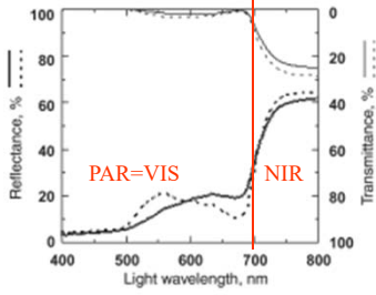
Figure 3. Reflectance (bold lines) and transmittance (thin lines) of light (400–800 nm) by young Planchonella obovata var. dubia leaves with (solid lines) and without (dashed lines) epidermal leaf hairs. Ishida et al. (2001: Tree Physiology 21, 497)
