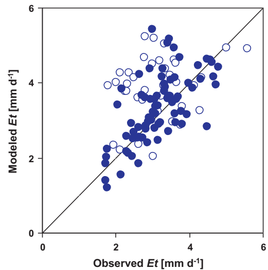
Fig. 5. Relationship between observed transpiration ( Et ) and modeled results under dry canopy conditions. The modeled Et is the average of maximum and minimum estimates. The solid line indicates observed Et = modeled Et . The data were differentiated with soil moisture condition; ● >50 mm, ○ <50 mm.
